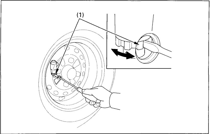
(1) Brake adjusters
