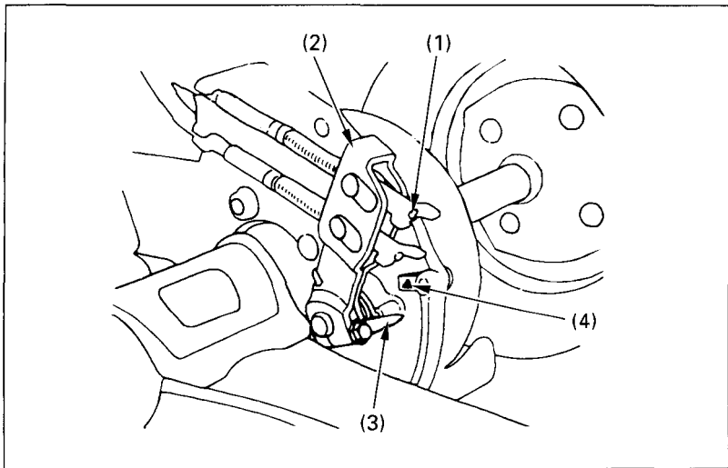
Fig. 4-29 (1) Brake lever adjusting nut (3) Arrow (2) Brake arm (4) Reference mark
