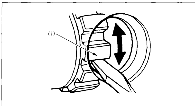
(1) Brake adjuster
