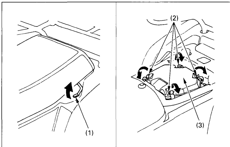
Fig. 4-5 (1) Seat lock lever (2) Retainer clips
