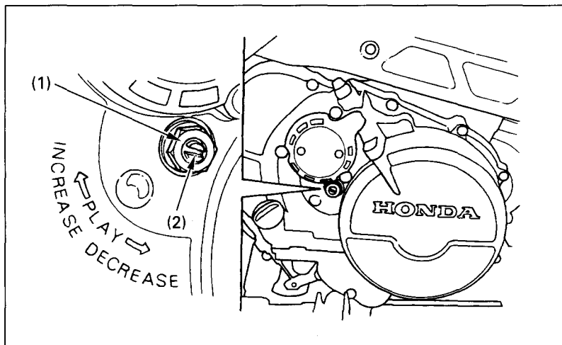
Fig. 4-17 (1) Lock nut
