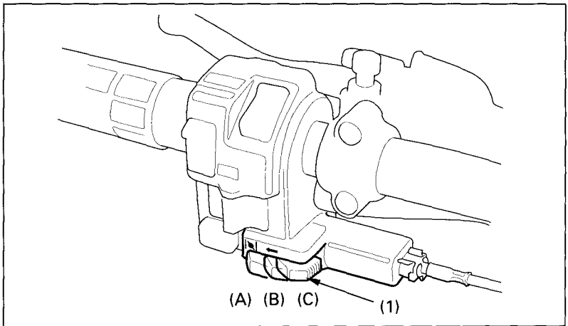
Fig. 3-9 (1) Choke lever
