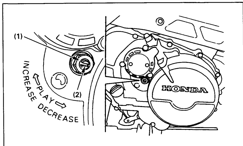
(2) Clutch adjuster
