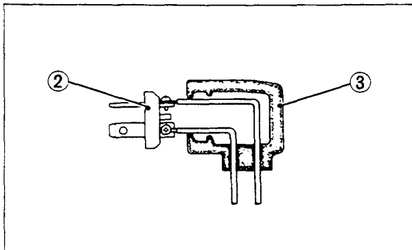
(2) Special plug
