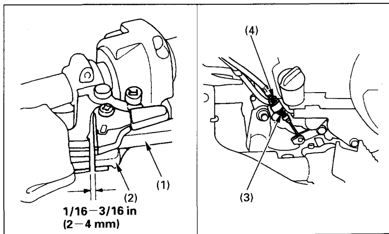
(3) Lock nut (4) Adjusting nut
