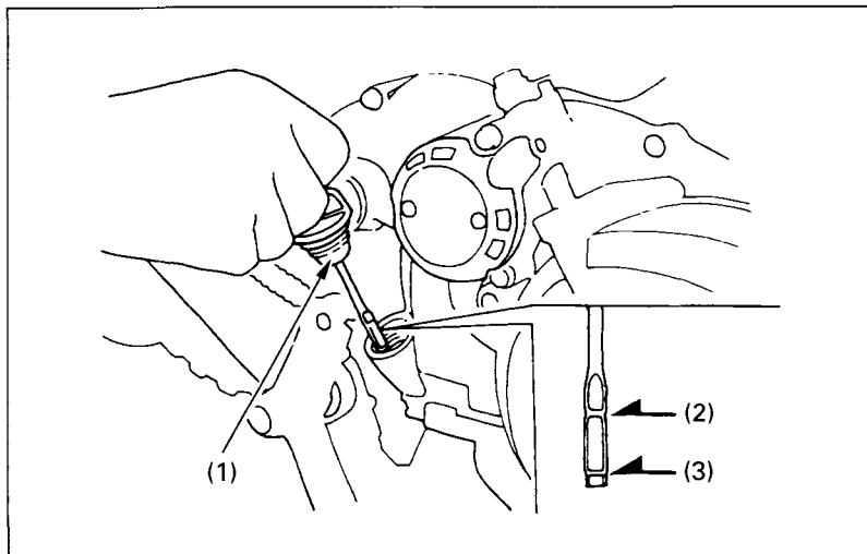
Fig. 2-19 (1) Oil filler cap/dipstick
