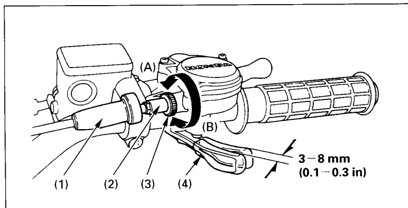
Fig. 4-4 (1) Rubber sleeve (2) Cable adjuster (3) Lock nut (4) Throttle lever (A) To decrease free play (B) To increase free play
