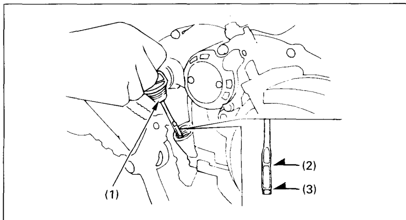
Fig. 4-10 (1) Oil filler cap/dipstick (2) Upper level mark
