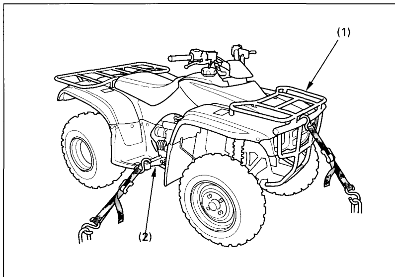
Fig. 4-36 Points to secure FOURTRAX with tie downs
