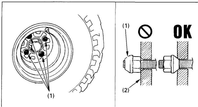
Fig. 4-30 (1) Wheel nuts
