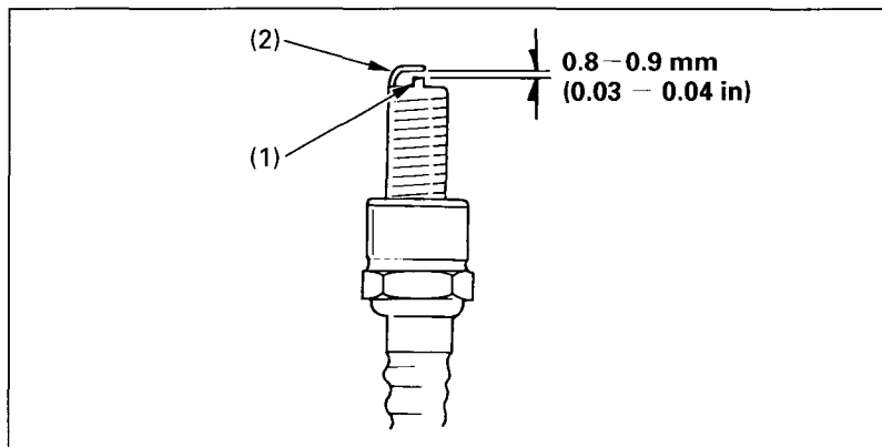
Fig. 4-14 (1) Center electrode (2) Side electrode
