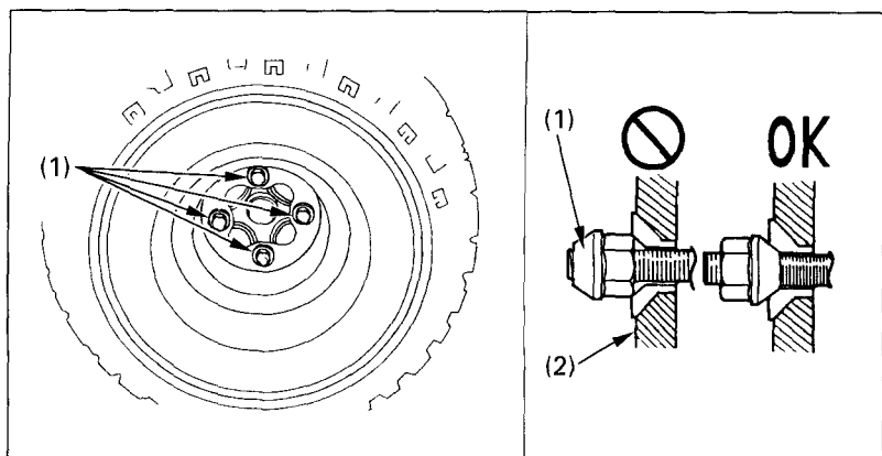
Fig. 4-27 (1) Wheel nuts
