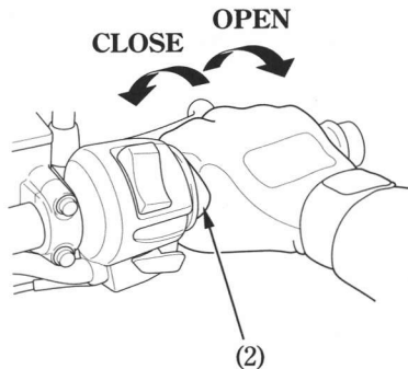
(2) Throttle
