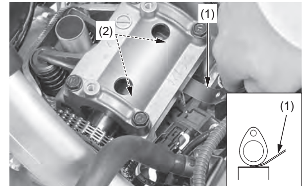
(1) feeler gauge (2) valve lifters and cam lobes
