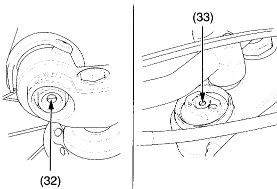
(32) rebound damping adjuster screw
