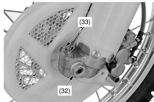
(32) front axle nut (33) left axle pinch bolts
