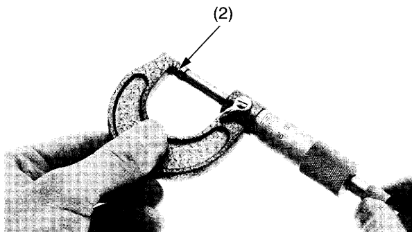
(2) shim
