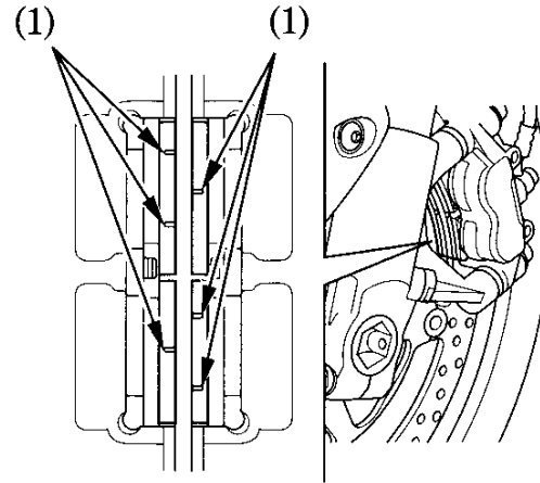
(1) Wear indicator grooves
