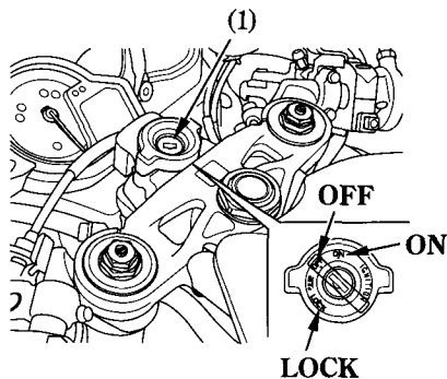
(1) Ignition switch
