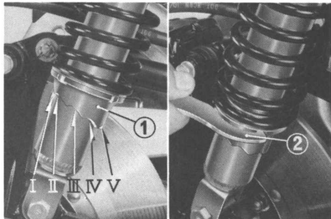
(1) Rear shock absorber (2) Pin spanner
