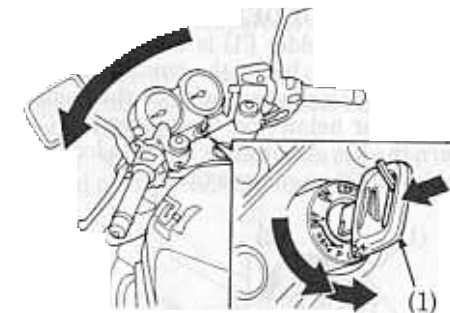
(1) Ignition key
