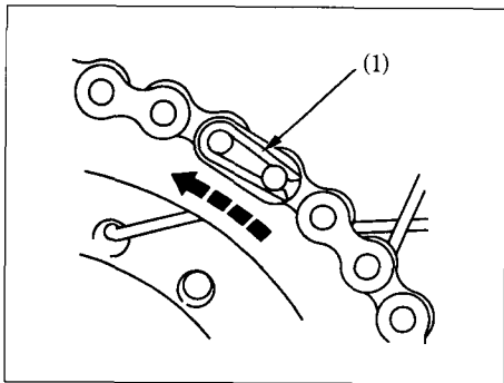
(1) Retaining clip
