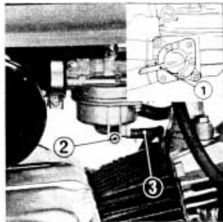
① Fuel valve ② Drain screw ③ Drain tube
